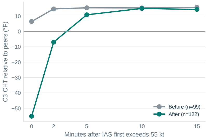
C3 catches up after power is applied
