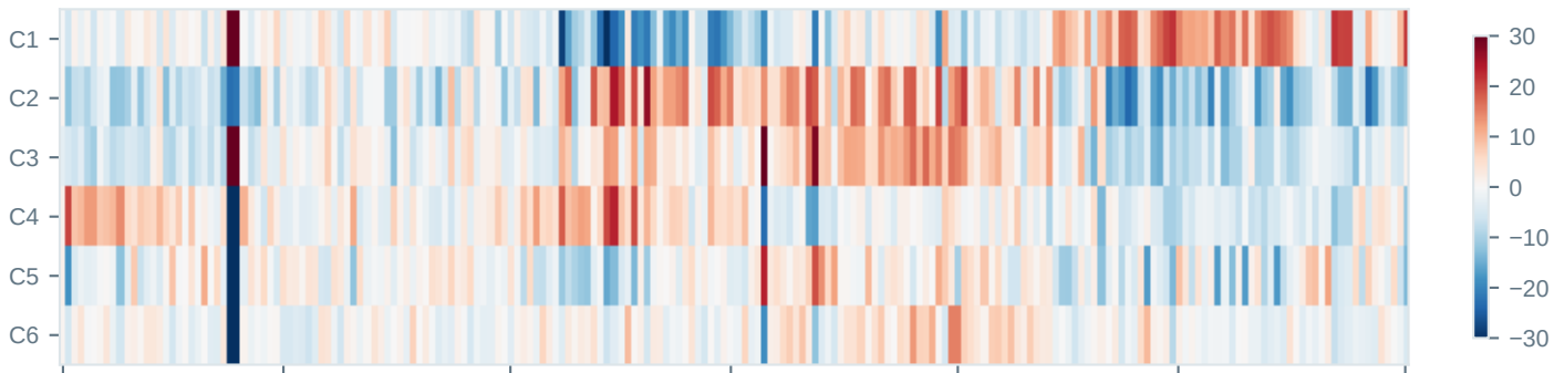
CHT differential vs similar flights (°F)
